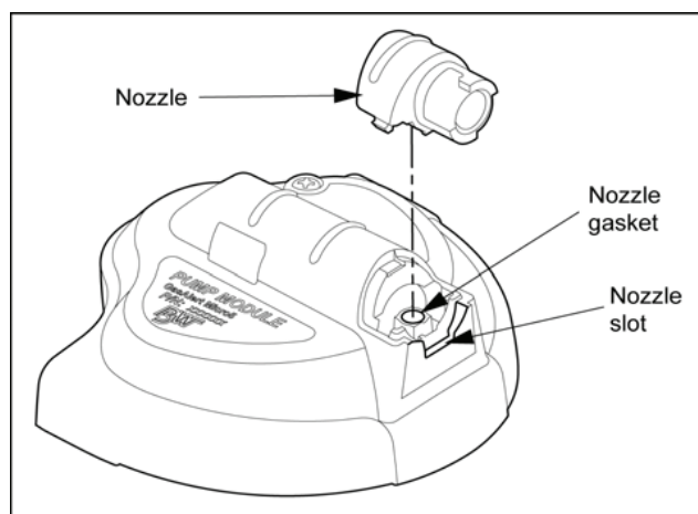
Figure 8. Replacing the Pump Nozzle
