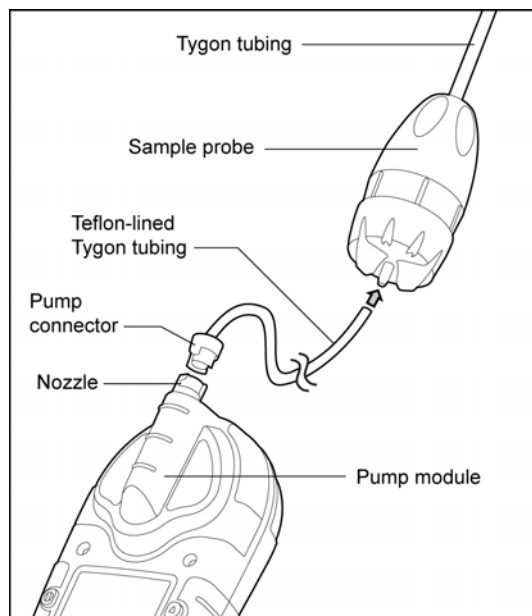
Figure 11. Attaching the Sample Probe
