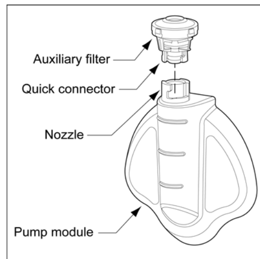
Figure 9. Attaching the Auxiliary Filter
