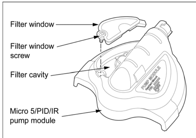
Figure 7. Replacing the Pump Filter
