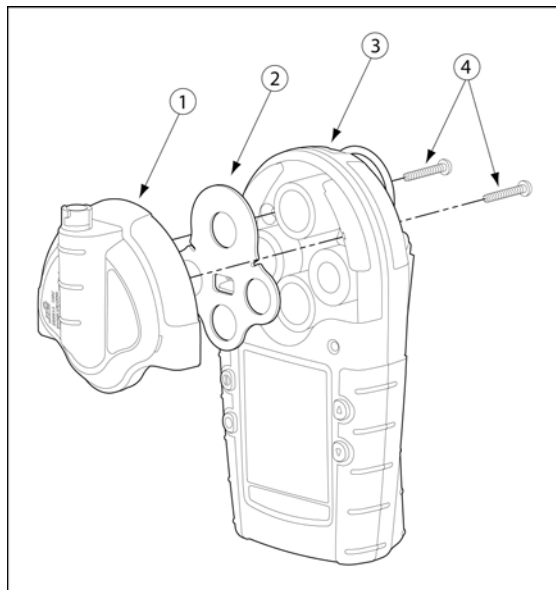
Figure 6. Installing the Pump Module
