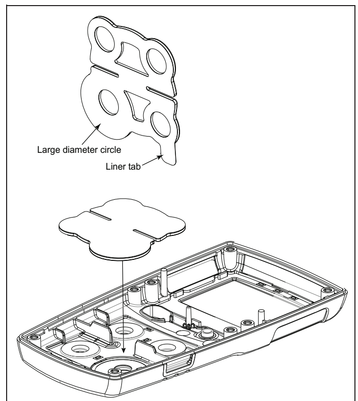
Figure 10. Liner Tab
