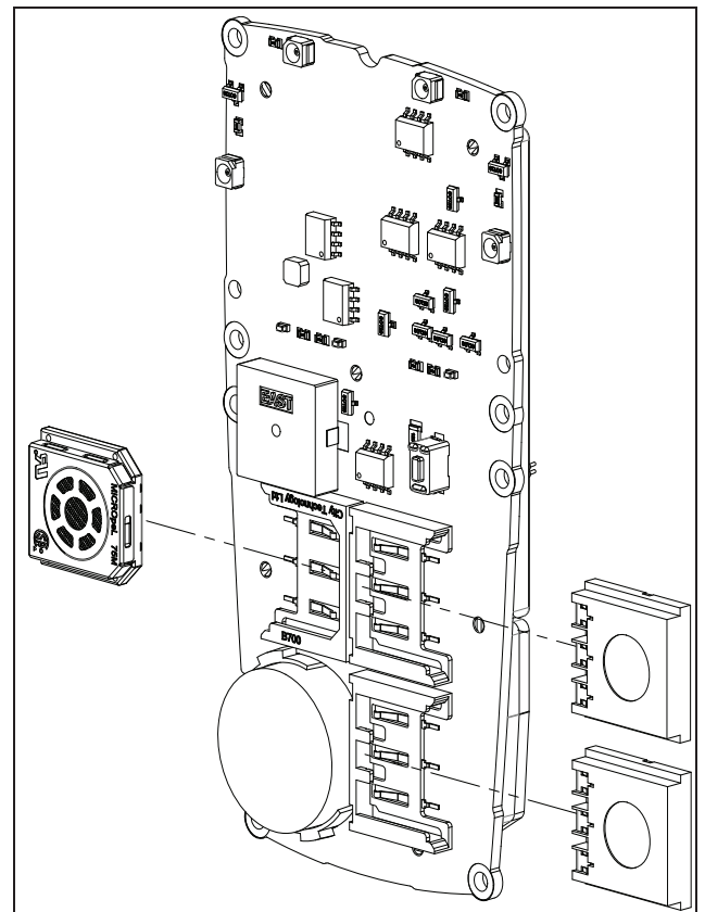
Figure 11. Sensor Positioning
