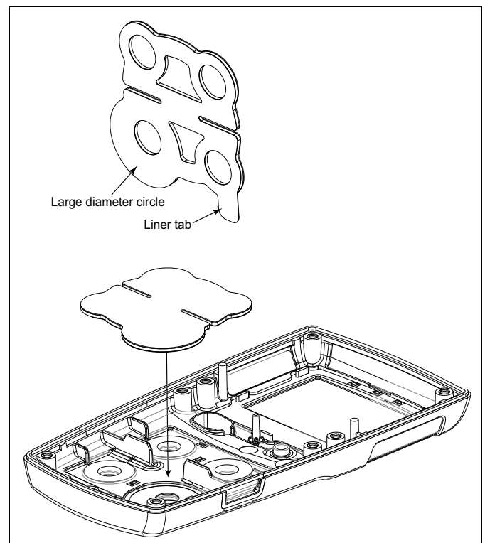
Figure 10. Liner Tab
